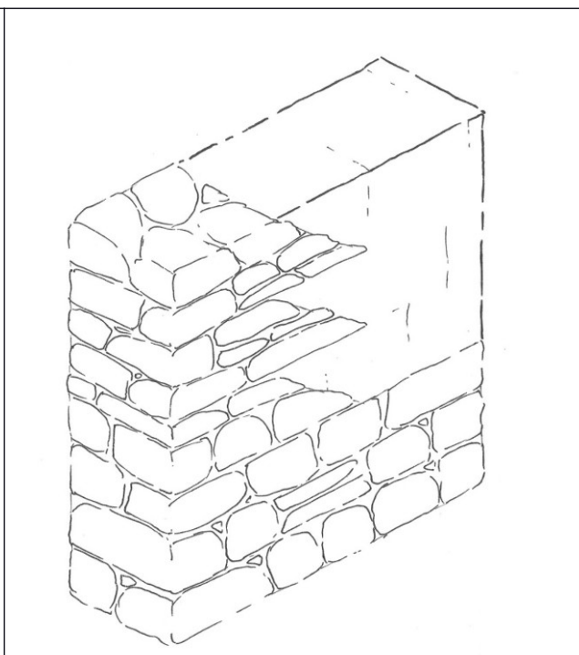
Figure 21: Jonction pierre/bauge
