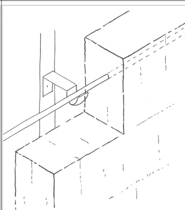
Figure 23: Liaison souple
